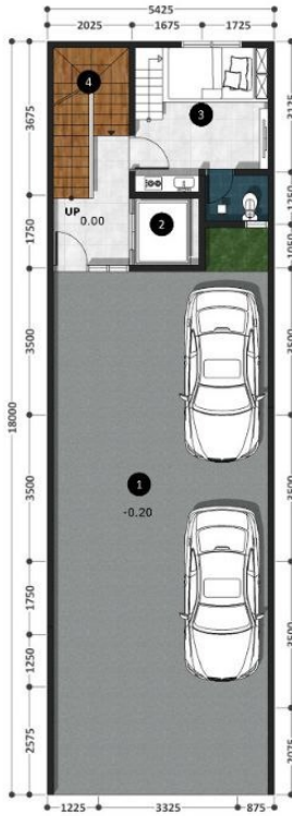
DENAH LANTAI 1
