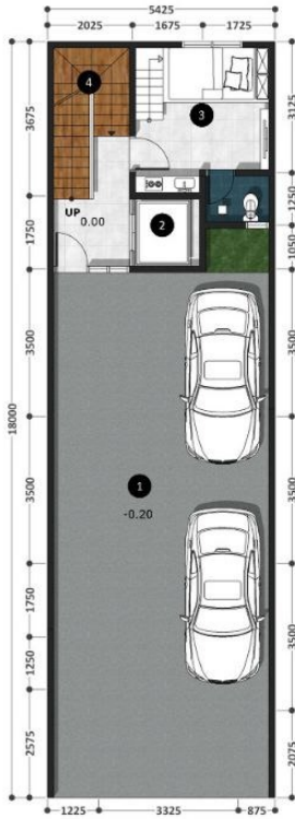
DENAH LANTAI 1
