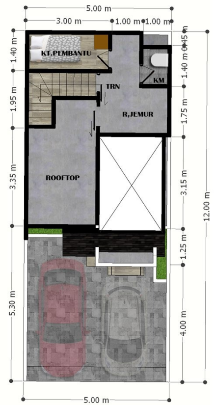
DENAH LANTAI 3
