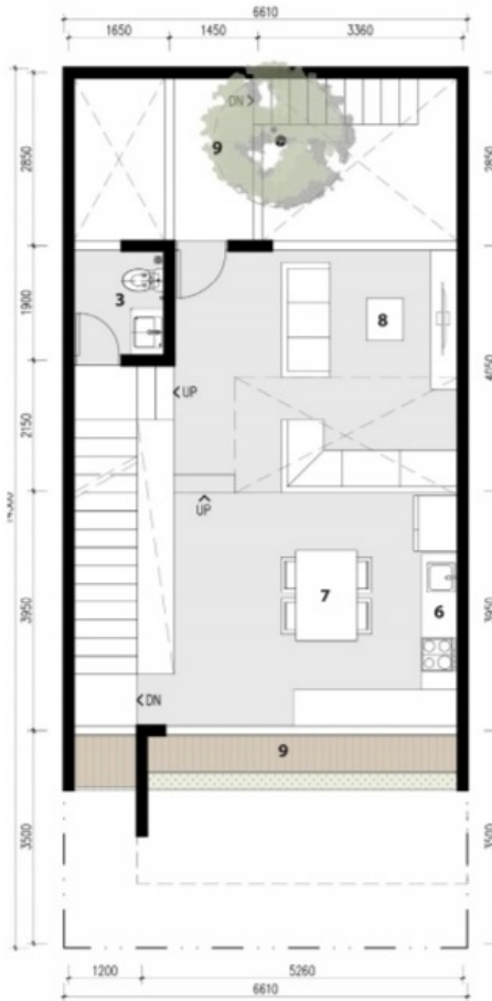
1st FLOOR
