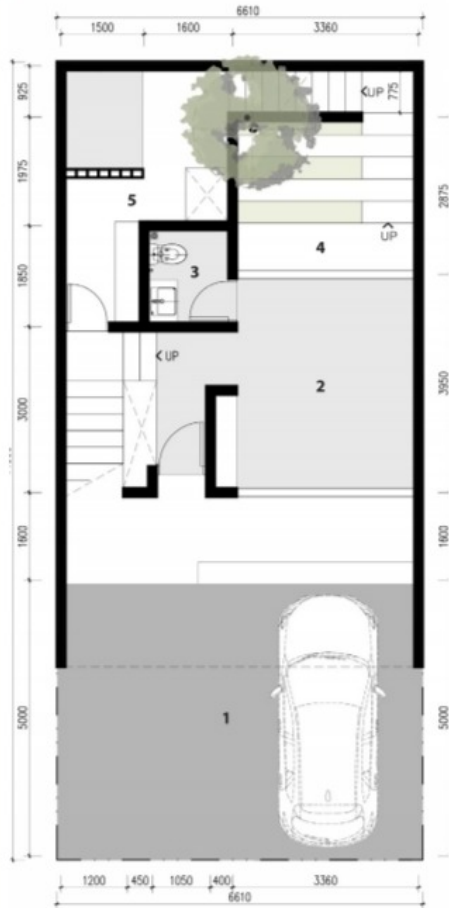
GF FLOOR
