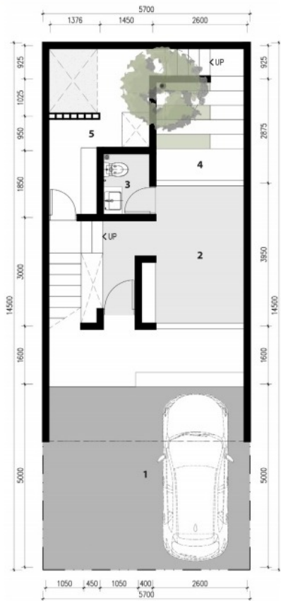
GF FLOOR
