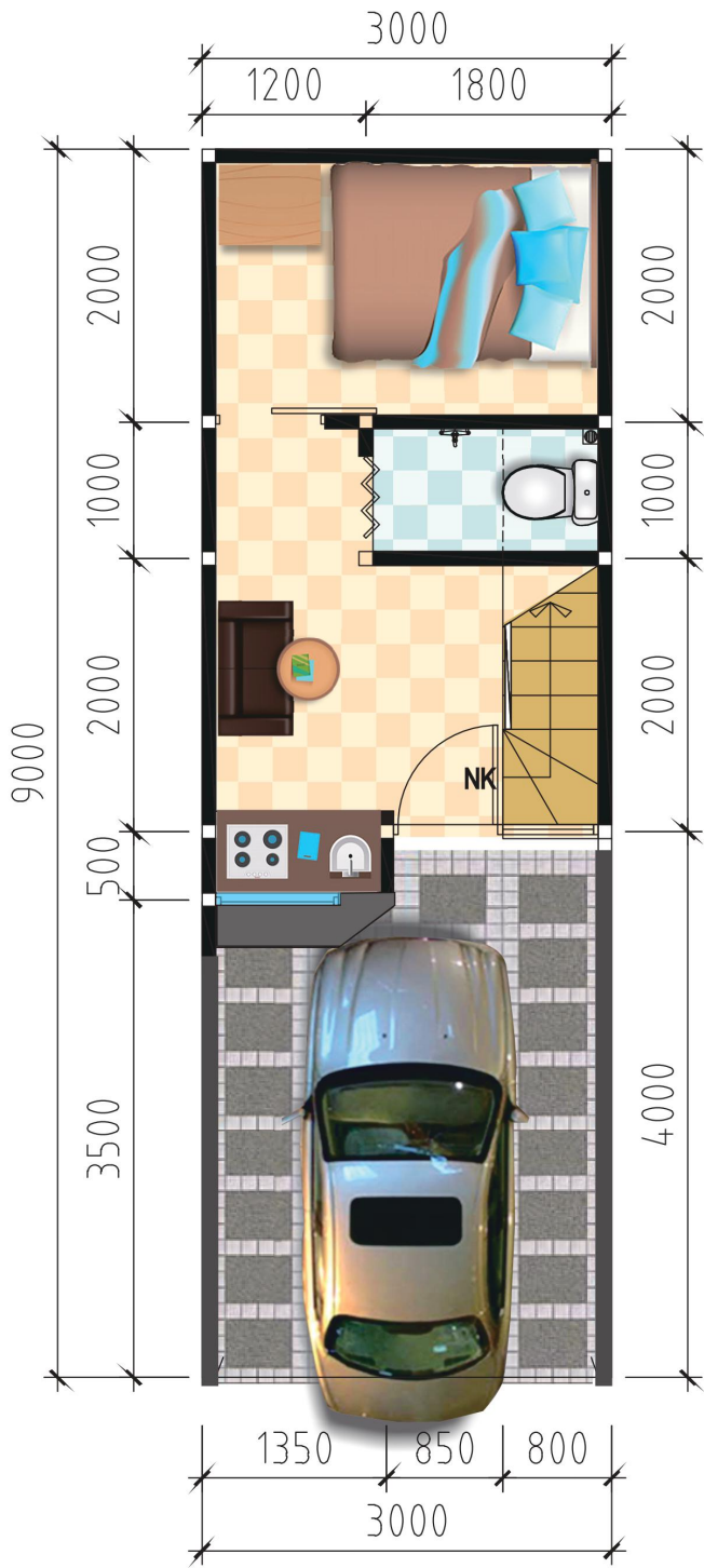
DENAH LANTAI 1
