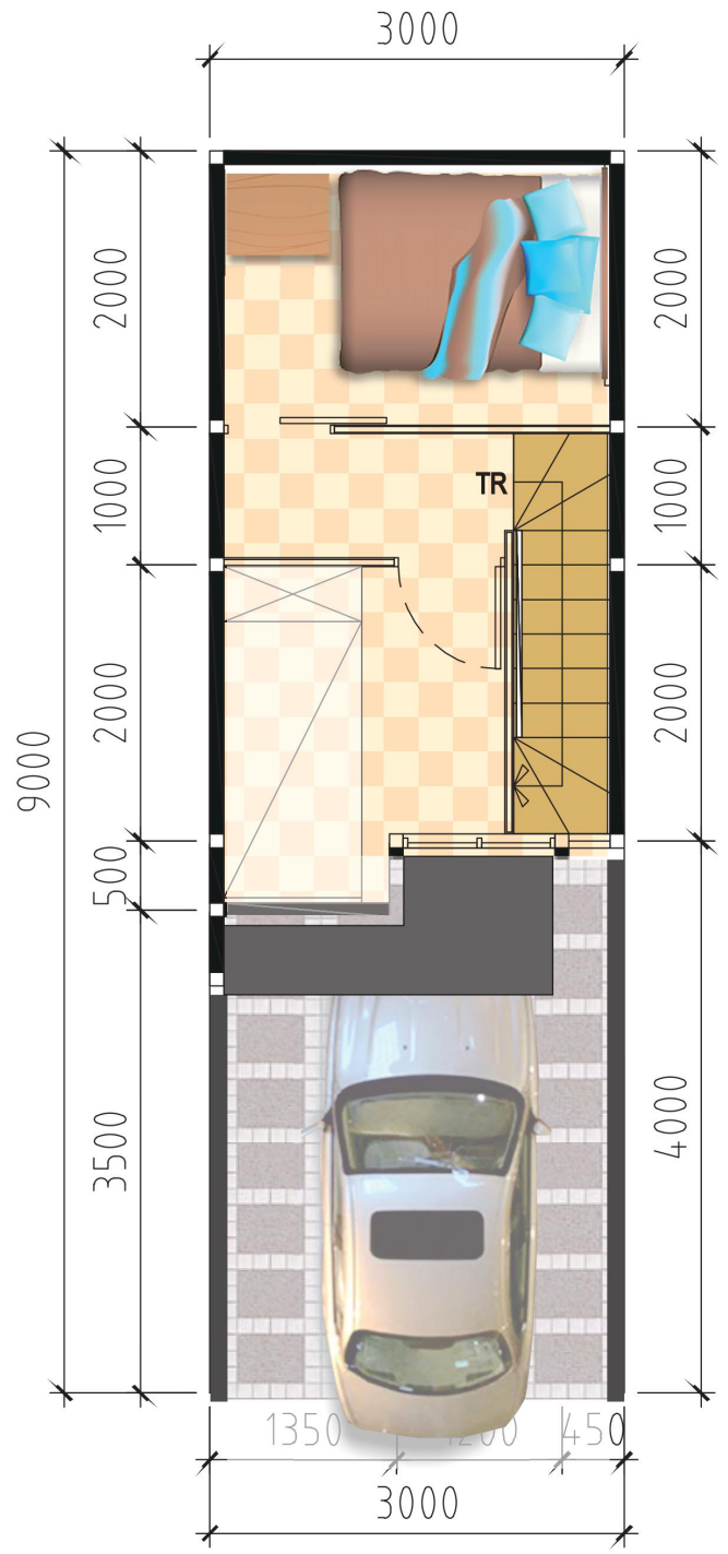
DENAH LANTAI 2
